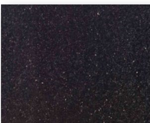
Star Galaxy
